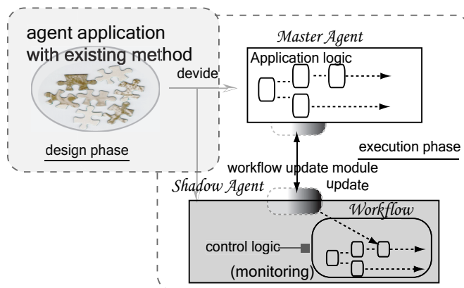
Fig. 2. Concise descriptions of WFA. At the design phase, an old-style agent application is divided into MA and SA. At the execution phase, workflow instance is kept fresh.
