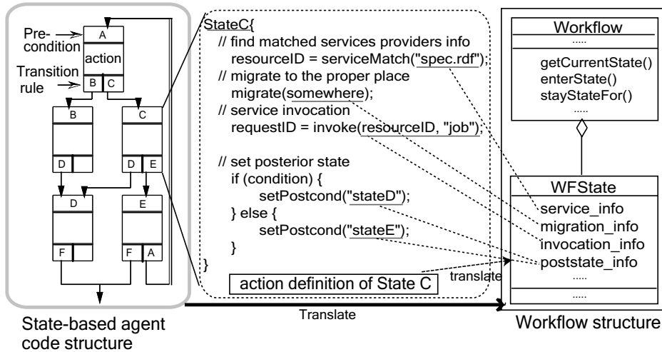
Fig. 3. Translation processes of an agent code. Each state of an agent code is translated into WFState, which becomes a workflow object's component. In this figure, state C is used as example. Potential workflow elements (method arguments) are extracted into WFState.
